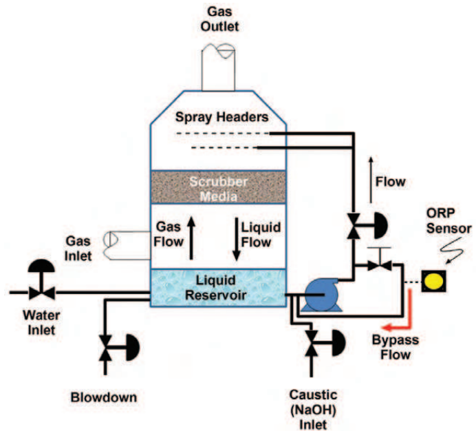
Figure 2. Chlorine gas scrubber controlled by ORP.
